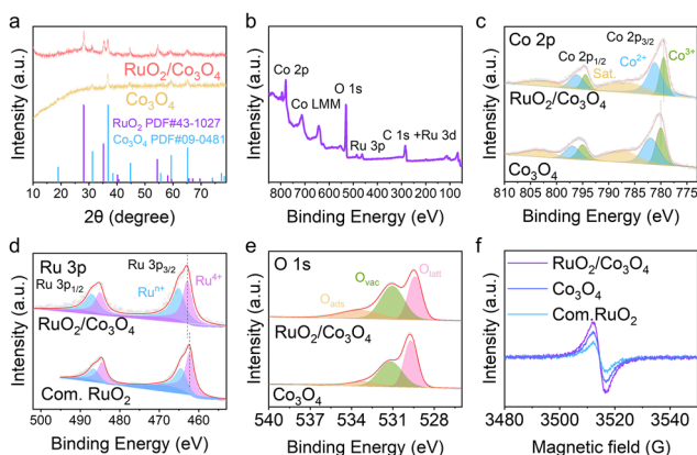
Fig. 3 (a) XRD patterns of \text{RuO}_2/\text{Co}_3\text{O}_4 and \text{Co}_3\text{O}_4 . (b) The whole XPS spectra of \text{RuO}_2/\text{Co}_3\text{O}_4 . (c)–(e) The XPS spectra of (c) Co 2p, (d) Ru 3p, and (e) O 1s for \text{RuO}_2/\text{Co}_3\text{O}_4 . (f) Electron paramagnetic resonance of \text{RuO}_2/\text{Co}_3\text{O}_4 , com. \text{RuO}_2 and \text{Co}_3\text{O}_4 .
