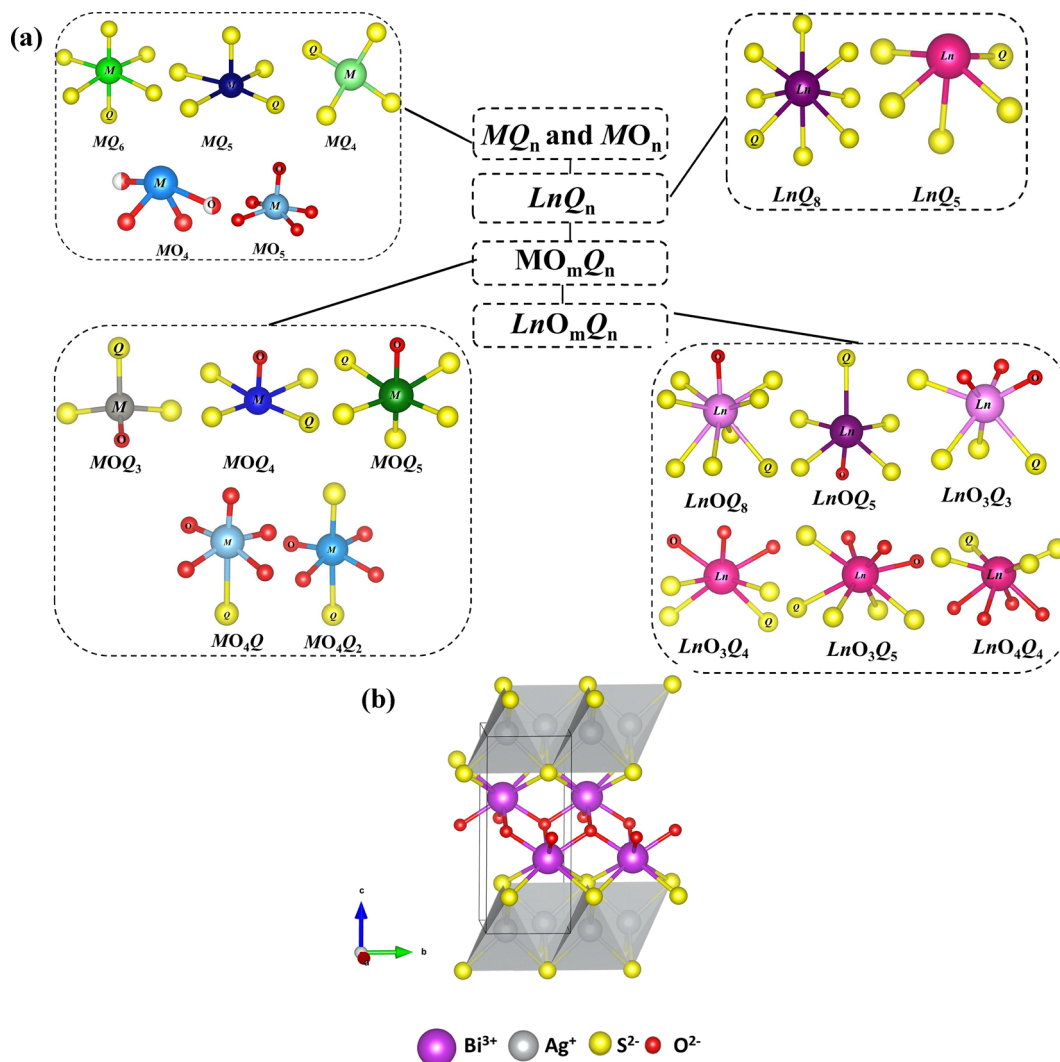
Fig. 2 (a) Schematic summarizing some coordination environments in oxychalcogenides. (b) Example of the ZrCuSiAs structure packing motifs from panel 1, adopted by BiCuOQ , BiAgOQ and LnFeAsO (as discussed in Section 2.2.8).
