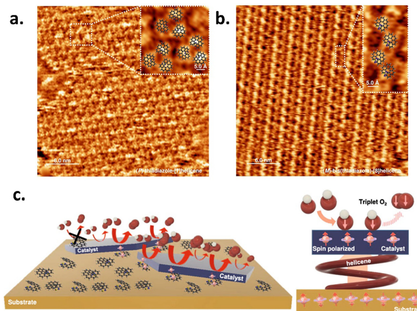
Fig. 3 Chirality-driven modulation of \text{NiO}_x electrocatalysts: STM image of SAM of (a) ( P )-thiadiazole-[7] helicene and (b) ( M )-bis(thiadiazole)-[8] helicene. (c) Illustration of the effect of spin polarization employing the catalyst-chiral molecule-Au substrate configuration. The figure is adopted from ref. 18 with permission from Nature © 2022.
