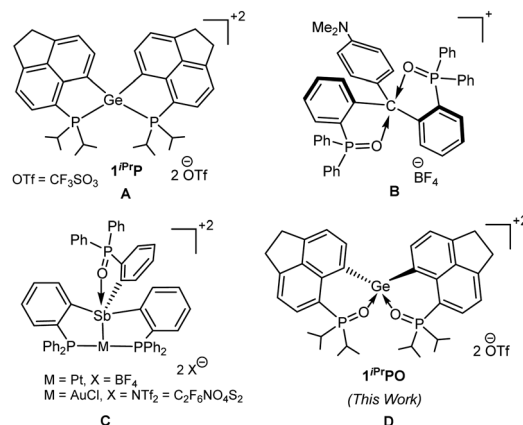
Fig. 1 (A) 1^{\text{IPr}} ; (B) phosphine-oxide stabilized triaryl carbenium ion; (C) phosphine-oxide stabilized Sb(V) di-cation; and (D) 1^{\text{IPr}}\text{PO} (this work).
