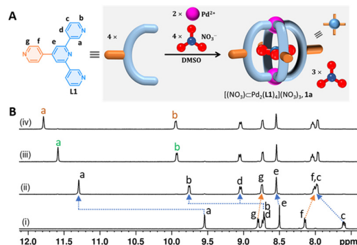
Fig. 1 (A) Schematic for the stoichiometry-controlled synthesis of a building block cage, 1a ; (B) ^1\text{H} NMR spectra of (i) ligand L1 , (ii) isolated \text{NO}_3^- cage 1a , and (iii)/(iv) halide-encapsulated cages obtained upon addition of 1 equiv. of TBACl/TBABr to 1a .
