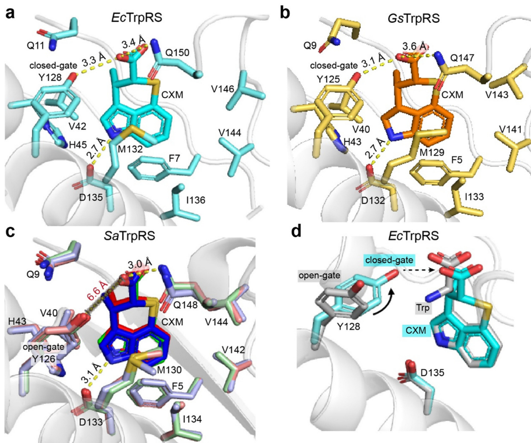
Fig. 3 Interactions between CXM and TrpRS across species. (a) EcTrpRS/CXM complex. (b) GsTrpRS/CXM (PDB: 7CMS, chain A). (c) SaTrpRS/CXM, with chains A, B, and C colored red, green, and blue, respectively. The distance between Y126 and CXM carboxylate (6.6 Å) indicates the lack of hydrogen bond with Y126. (d) Structural comparison of the EcTrpRS/CXM complex (cyan) and the EcTrpRS/Trp complex (gray; PDB: 8I4I, chain A). In the CXM complex, Y128 adopts a “closed-gate” conformation, with its phenol group oriented toward the ligand in the Trp-binding pocket. In contrast, Y128 in the Trp complex adopts an “open-gate” conformation, with its phenol group oriented away from the Trp-binding pocket.
