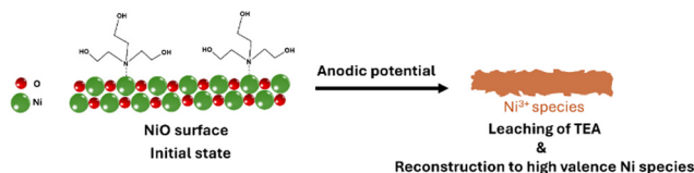
Fig. 5 Proposed transformation of the electrode surface of Ni/CP-TEA during the OER.
