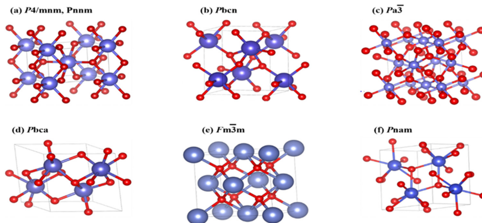
Fig. 5 Bulk formations of SnO 2 polymorphs, with blue and red representing Sn and O atoms, respectively. (a) Rutile in the P42/mnm and CaCl 2 -type in the Pnnm space groups, (b) R-PbO 2 -type in the Pbcn space group, (c) pyrite-type in the Pa3h space group, (d) ZrO 2 -type in the Pbca space group, (e) fluorite-type in the Fm3m space group, and (f) cotunnite-type in the Pnam space group.
