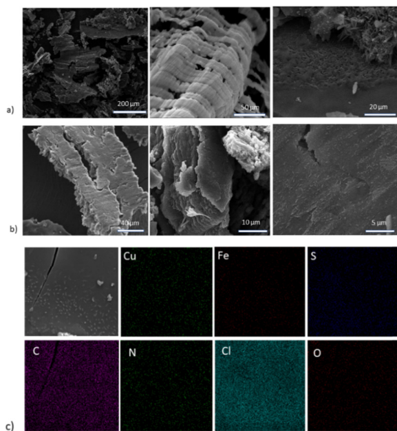
Fig. 3 SEM images of the (1–1) (a) bCOF@ \text{CuFeS}_2\text{--SDS} and (b) exfCOF@ \text{CuFeS}_2\text{--SDS} hybrid materials. (c) EDX mapping of the Cu, Fe, and S elements of the nanoparticles on bCOF@ \text{CuFeS}_2\text{--SDS} .
