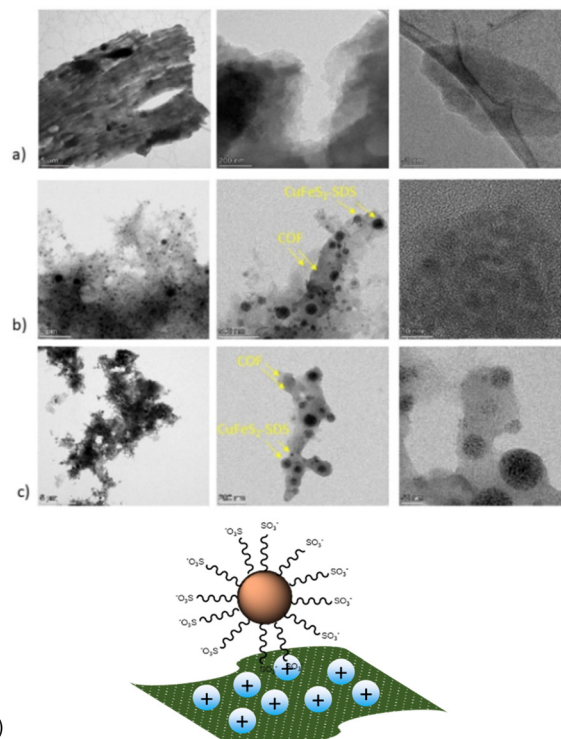
Fig. 4 TEM images of (a) bCOF, (b) (1–1) bCOF@ \text{CuFeS}_2\text{--SDS} and (c) (1–1) exfCOF@ \text{CuFeS}_2\text{--SDS} (d) and a schematic representation of the as-formed hybrids.
