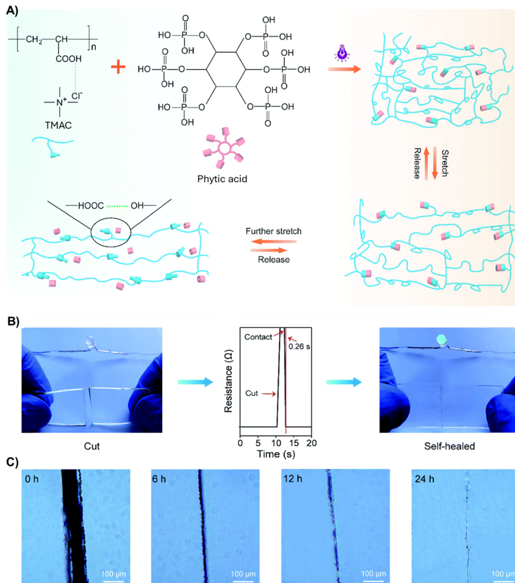
Fig. 4 (A) Schematic illustration of the extremely tough and ultra-stretchable polyDES based on TMAC, AA, and phytic acid molecules. (B) Digital images of the electrical self-healing process for a broken ICE in series with an LED. The film's resistance could recover rapidly to its original value without external stimuli within 0.26 s. (C) Optical microscope images of the self-healed ICE (10 wt% phytic acid) at room temperature for 24 h. Adapted from ref. 72 with permission from the Royal Society of Chemistry.
