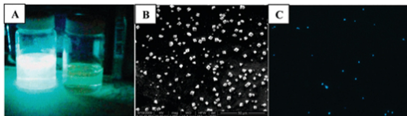
Fig. 2 Above: Structure of compound 1 (left), emission spectra of compound 1 in acetone–water mixtures; concentration = 10 \mu M, \lambda_{exc} = 360 nm (right). Below: (A) image of compound 1 taken in an acetone–water (40 : 60 v/v) mixture (left) and in pure acetone (right) under 365 nm UV light. (B) SEM image of compound 1 in an acetone–water (40 : 60 v/v) mixture. (C) Fluorescence microscopy image of microcrystals of compound 1 in an acetone–water (40 : 60 v/v) mixture. Reproduced with permission from ref. 70. Copyright 2011 the American Chemical Society.
