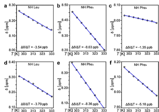
Fig. 2 Intramolecular H-bonds in the heterochiral tetrapeptide. Variable-temperature ^1\text{H-NMR} analysis of CONH signals in DMSO (a)–(c) and with 20% water (d)–(f). Note: higher amounts of water led to precipitation.
