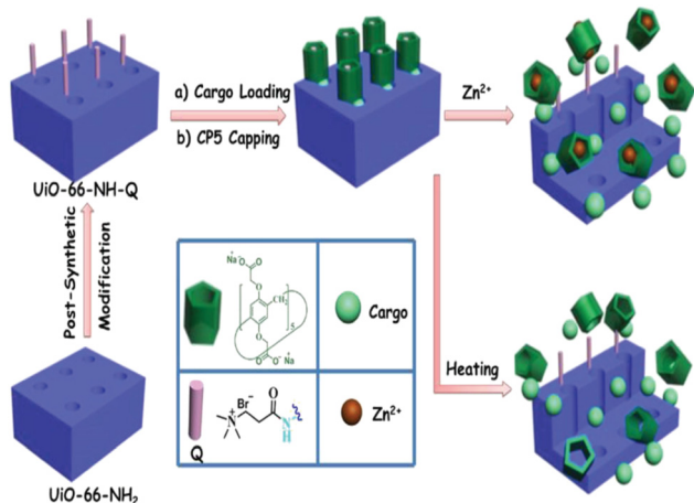
Fig. 4 Schematic representation of stimuli-responsive mechanized UiO-66-NH 2 MOFs equipped with positively charged quaternary ammonium salt (Q) encircled by pillarane [2]pseudorotaxanes. The mechanized nanoUiO-66-NH 2 MOFs can be operated either by thermal heating or by Zn 2+ competitive binding in regulation of the release of cargo molecules. Reproduced from ref. 62 with permission from Royal Society of Chemistry, copyright 2015.
