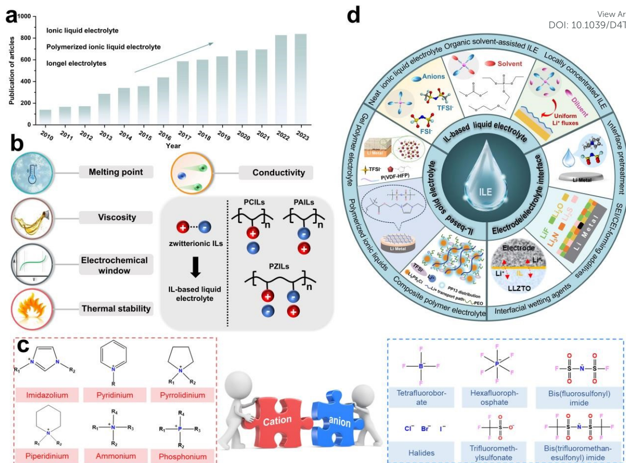
Fig. 1 (a) Number of publications of ionic liquids applied in batteries. Data are obtained from Web of Science on the 30th May, 2024, via keyword of ionic liquid electrolyte, polymerized ionic liquid electrolyte and iongel electrolyte. (b) The key parameters for evaluating ionic liquid as electrolytes. (c) Chemical structures of various ILs. (d) Summary of ionic liquid application.
