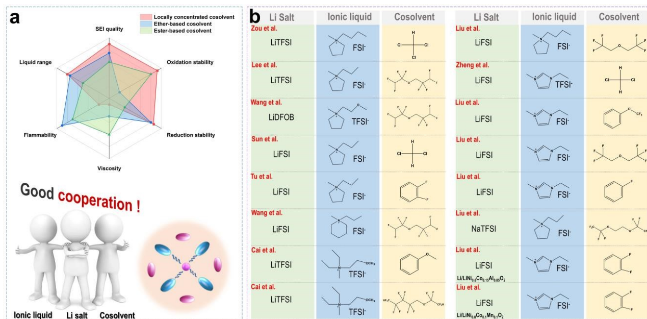
Fig. 7 (a) Comparison of the physicochemical and electrochemical properties of ILE using ether-based cosolvent, ester-based cosolvent, and locally concentrated cosolvent in radar chart; and classical LCILE solvation structure. (b) Summary of the combination and collocation of LCILE composed of lithium salt, cosolvent and ILs.
