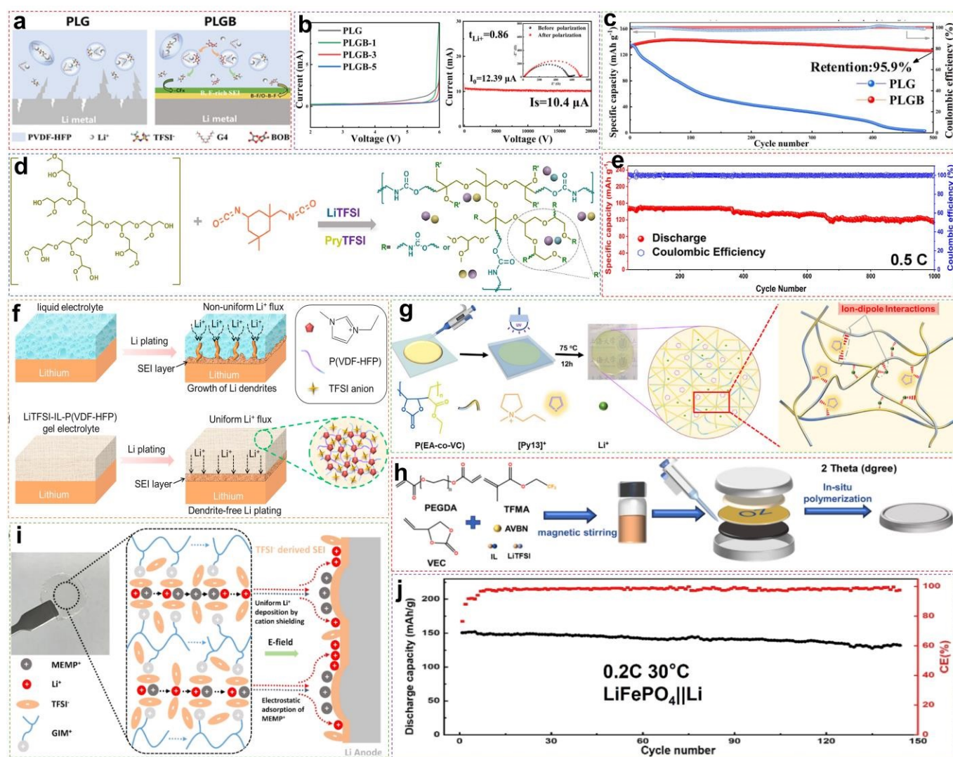
Fig. 11 (a) Schematic representation of Li + transport in PLG and PLGB GPE. (b) The LSV measurement of SS/GPE/Li batteries and DC polarization profiles of the symmetrical Li/PLGB/Li battery (the inset shows the impedance spectra before and after polarization). (c) A comparison of the long-term cycle performance between LFP/PLG/Li and LFP/PLGB/Li batteries at 0.5 C. Reproduced from ref. 107 with permission. Copyright 2023, The Royal Society of Chemistry. (d) Schematic diagram of HPU-based electrolyte. (e) Cycling performance of LFP/HPU1.5-IL1.5/Li cell at 0.5 C and RT. Reproduced from ref. 108 with permission. Copyright 2024, Elsevier. (f) Schematic illustration of the electrochemical deposition behavior of lithium metal anodes with liquid organic solution electrolyte and LiTFSI-IL-P(VDF-HFP) gel electrolyte. Reproduced from ref. 110 with permission. Copyright 2018, Elsevier. (g) Schematic diagram for the preparation of CLSPE-IL. Reproduced from ref. 111 with permission. Copyright 2022, Elsevier. (h) In situ thermal curing battery assembly flow chart. Reproduced from ref. 112 with permission. Copyright 2024, Elsevier. (i) Schematic illustration of GM-GPE that enhances ionic transport and stabilizes the GPE/Li anode interface. (j) Cycling performances of the LFP/GM-GPE/Li cell at 30 °C. Reproduced from ref. 91 with permission. Copyright 2024, American Chemical Society.
