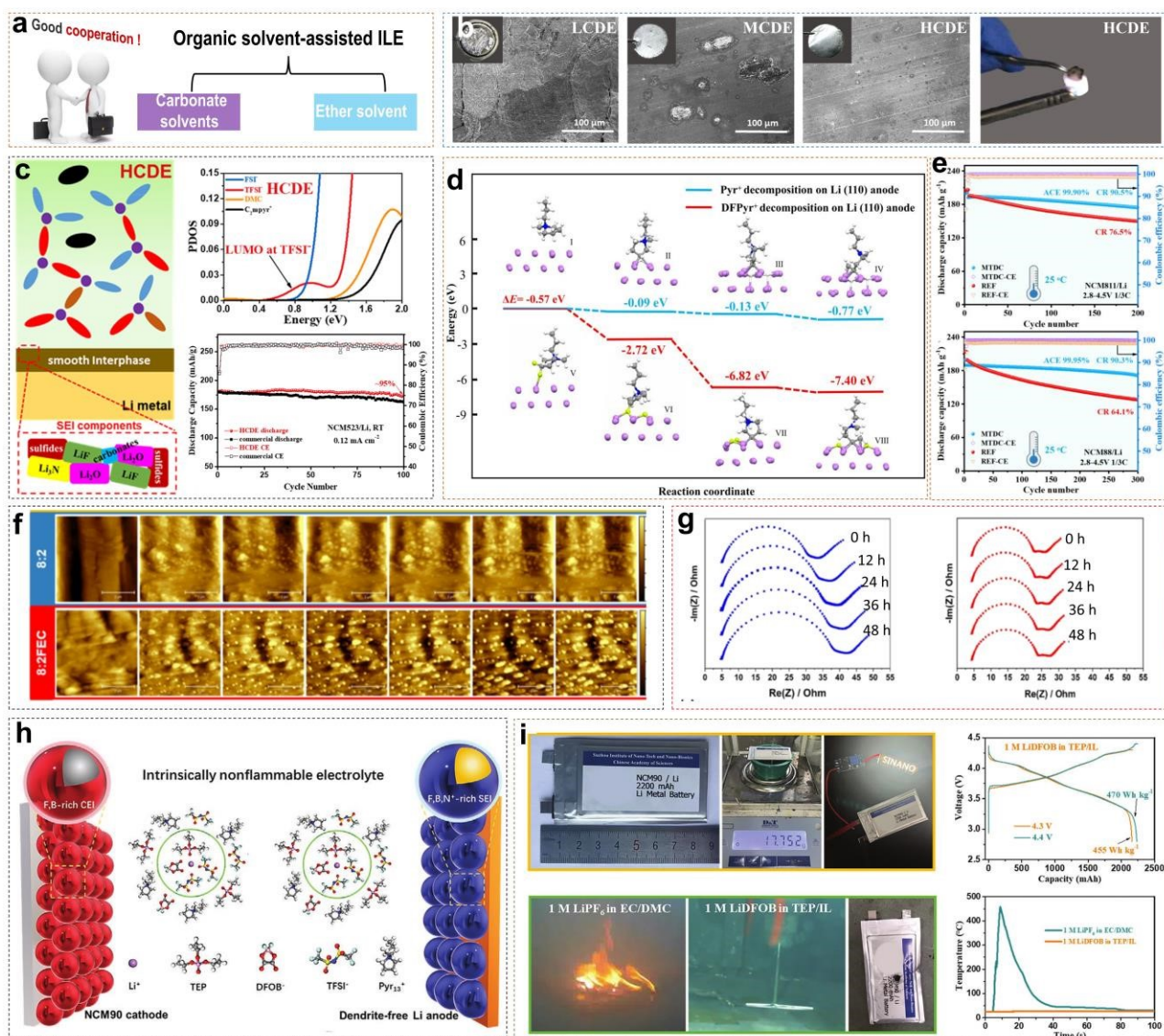
Fig. 5 (a) Classification of organic solvents for organic solvent-assisted ILE. (b) Corrosion of Al foil in different electrolytes and combustion tests of HCDE. (c) Schematic of the SEI formed on the LMA surface and PDOS obtained by DFT calculations with HCDE; corresponding cycling performance of Li/NCM523 LMBs. Reprinted from ref. 40 with permission. Copyright 2020, Elsevier. (d) Reduction pathway of difluorinated IL on Li metal. (e) Cycling stability and Coulombic efficiency of Li/NCM811 and Li/NCM88 cells under 2.8-4.5 V cutoff voltage at 25 °C. Reprinted from ref. 41 with permission. Copyright 2023, Wiley. (f) In situ AFM mappings (area 5 \times 5 \mu\text{m}^2 ) of lithium plated onto nickel current collectors at 80 \mu\text{A cm}^{-2} employing 8:2, and 8:2:FEC as the electrolyte. (g) EIS performed on \text{Li}_n/\text{Li} cells using 8:2 and 8:2:FEC during a two-day rest period with spectra recorded every 12 h. Reprinted from ref. 43 with permission. Copyright 2023, American Chemical Society. (h) Schematic diagram of the Li/NCM90 LMBs and solvation structure with the intrinsically non-flammable electrolyte. (i) Nail penetration test, charge/discharge curves and temperature versus time of the Li/NCM90 pouch cells. Reprinted from ref. 44 with permission. Copyright 2023, Wiley.
