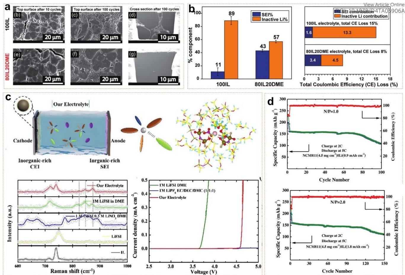
Fig. 6 (a) Morphology of top surface and cross-section by Cryo-FIB in 100IL and 80IL20DME electrolyte. (b) Quantitative analysis of Li 0 inactive and Li + SEI by TGC quantification method. Reprinted from ref. 45 with permission. Copyright 2022, The Royal Society of Chemistry. (c) Schematically illustration of Li/NCM811 full cells in IL-based electrolytes; Raman spectra, and liner sweep voltammetry curves. (d) Cycling performance of Li/NCM811 full cell under N/P ratio of 2 and 1. Reprinted from ref. 46 with permission. Copyright 2023, Wiley.
