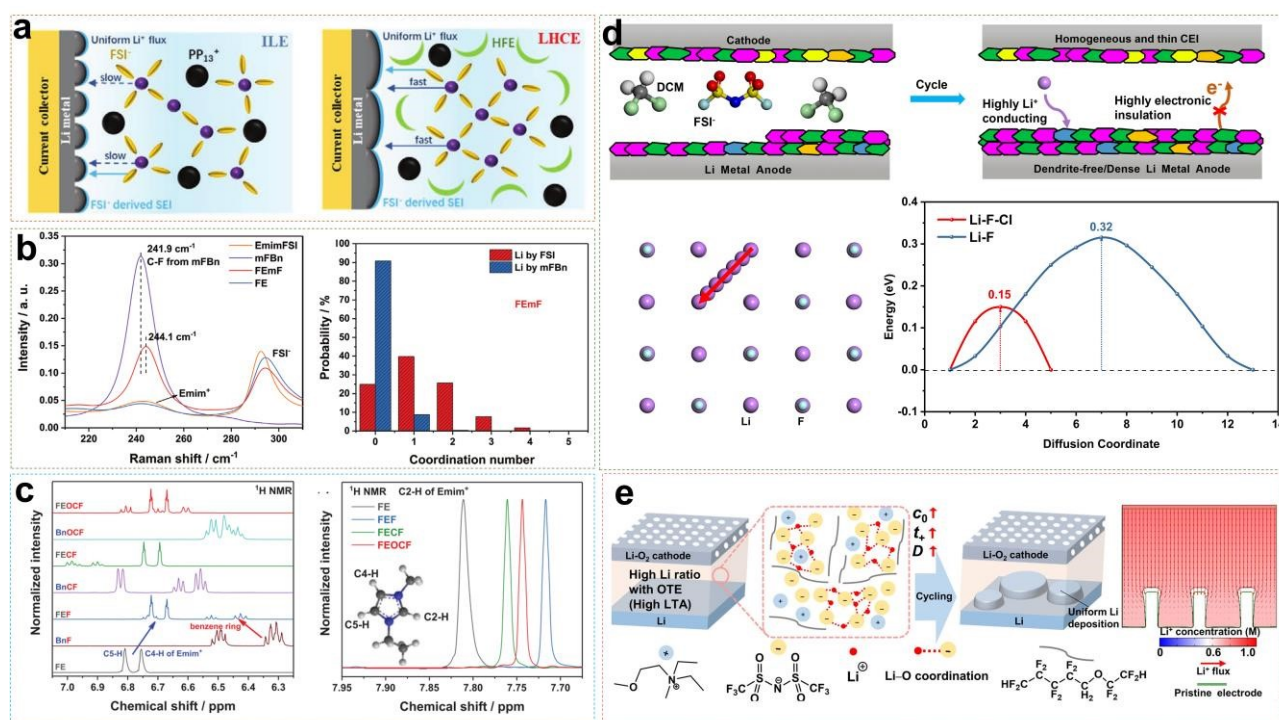
Fig. 8 (a) Schematic diagrams of Li plating on Cu current collector and solvation structure of ILE and LHCE. Reprinted from ref. 51 with permission. Copyright 2021, Wiley. (b) Li + ion solvation structure with mFBn and the corresponding Raman characterization and coordination number calculation. Reprinted from ref. 58 with permission. Copyright 2022, Wiley. (c) 1D 1 H NMR spectra of the electrolytes and their constituents in the region of 6.25-7.05 ppm and 7.675-7.950 ppm. Reprinted from ref. 59 with permission. Copyright 2023, Wiley. (d) Schematic illustrations of the SEI/CEI components from LCM systems and Li + diffusion path and migration energy barriers of Li + along LiF-LiCl grain boundaries. Reprinted from ref. 61 with permission. Copyright 2024, American Chemical Society. (e) Schematic diagram of Li deposition behavior by regulating T_{sand} with OTE. Reprinted from ref. 63 with permission. Copyright 2021, Wiley.
