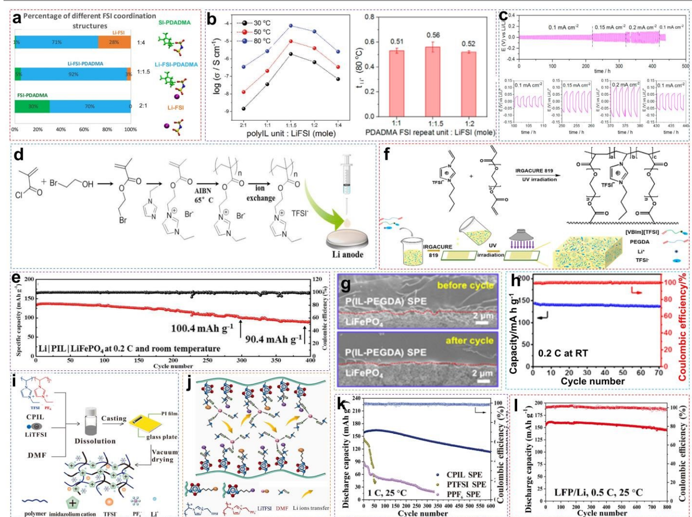
Fig. 10 (a) Percentage of anions in three types of FSI ^- coordination environment calculated from MD simulations at 353 K. (b) The ion conductivities of different polyLiL/salt systems at different temperatures and the \text{Li}^+ transference number of solid polymer electrolytes with varying polymer-to-salt ratios. (c) The Li/Li symmetric battery cycling performances of polymer electrolyte 1:1 at various current densities (i.e., 0.1, 0.15, and 0.2 \text{mA cm}^{-2} ). Reproduced from ref. 89 with permission. Copyright 2019, Elsevier. (d) Schematic representation of the synthesis of PIL. (e) Cycling performance of LFP/PIL/Li batteries at 0.2 C and RT. Reproduced from ref. 90 with permission. Copyright 2023, The Royal Society of Chemistry. (f) Schematic diagram of the P(IL-PEGDA) SPE copolymerization reaction and preparation process. (g) SEM image of the interface between LFP cathode and P(IL-PEGDA) SPE before and after 50 cycles. (h) Cycling performance of LFP/P(IL-PEGDA) SPE/Li batteries at 0.2 C and RT. Reproduced from ref. 92 with permission. Copyright 2020, American Chemical Society. (i) Schematic illustration of the fabrication of solid polymer electrolytes. (j) Schematic representation of \text{Li}^+ transfers in robust-flexible CPIL SPE. (k) Cycling performance of NCM811/CPIL SPE/Li batteries at 1 C and RT. (l) Cycling performance of LFP/CPIL SPE/Li batteries at 0.5 C and RT. Reproduced from ref. 84 with permission. Copyright 2024, Elsevier.
