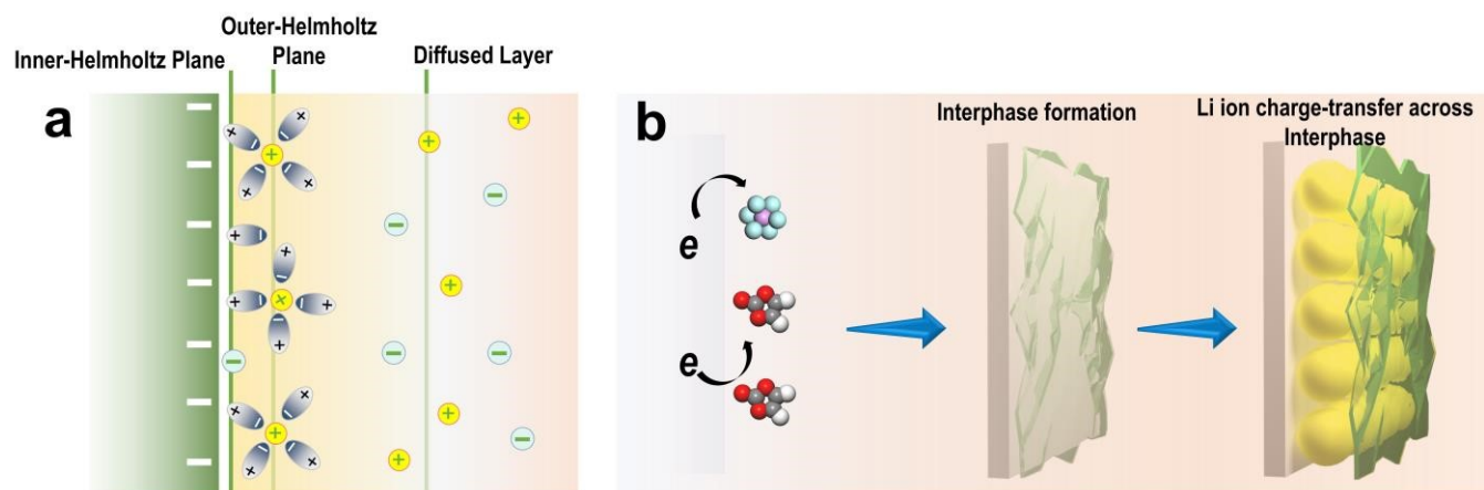
Fig. 13 (a) Schematic of electric double layer. (b) Illustration of the interphase formation and process of Li ion charge-transf
