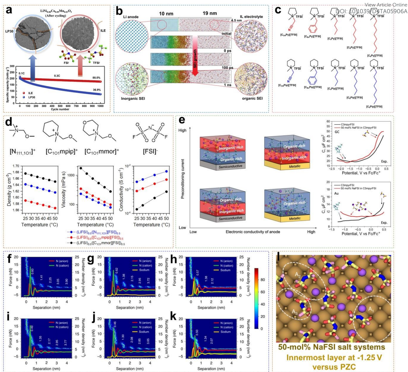
Fig. 3 (a) Long-term cycling performance of an exemplary Li/NCM88 cell using ILE and LP30 electrolyte. Reprinted from ref. 31 with permission. Copyright 2021, Elsevier. (b) The formation of the SEI layer from the ReaxFF MD simulation at 300 K using a [BMIM][TFSI] IL electrolyte. Reprinted from ref. 32 with permission. Copyright 2022, Wiley. (c) Chemical structures of pyrrolidinium- and piperidinium-based ILs. Reprinted from ref. 33 with permission. Copyright 2020, American Chemical Society. (d) Chemical structures and corresponding density, viscosity, and conductivity of different ether-functionalized ILEs. Reprinted from ref. 34 with permission. Copyright 2023, Elsevier. (e) Schematic relationships between the SEI composition, applied preconditioning current, and dielectric nature of the anode material. Reprinted from ref. 35 with permission. Copyright 2023, The Royal Society of Chemistry. (f-h) AFM force-distance two-dimensional histograms and ion number density profiles of FSI - , C 3 mpyr + and Na + from MD simulations at OCP (AFM) and PZC (MD) (f-h) and OCP -0.5 V (AFM) and -0.5 V versus PZC (MD) (i-k) for C 3 mpyrFSI IL with different NaFSI concentrations of 0 mol% (f, i), 10 mol% (g, j), and 50 mol% (h, k). (l) Typical Na-FSI coordination complexes in the innermost layer at -1.25 V versus PZC in the 50 mol% salt systems. Reprinted from ref. 36 with permission. Copyright 2020, Springer Nature.
