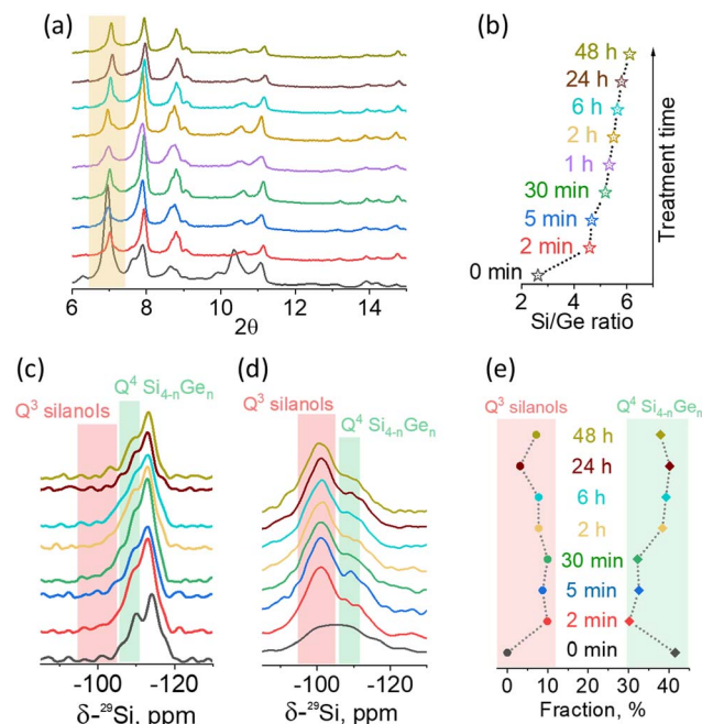
Fig. 2 Evolution of the structure, composition and state of framework atoms in OSDA-free UWY-2.6 zeolite (designated as “0 min”) treated with 6 \text{ M HCl} at RT for different times (2 min, 5 min, 30 min, 1 h, 2 h, 6 h, 24 h, and 48 h) followed by calcination. (a) XRD patterns (full patterns are shown in Fig. S8†). (b) \text{Si/Ge} ratio. (c) ^{29}\text{Si} MAS NMR spectra. (d) ^1\text{H}-^{29}\text{Si} CP MAS NMR spectra. (e) Population of \text{Q}^3 Si atoms in silanol groups (corresponding to the band at -103 ppm) and \text{Q}^4 Si atoms originating from D4R units (band at around -108 ppm). Fitting plots are shown in Fig. S10.†
