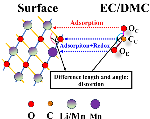
Fig. 5 Schematic diagram of decomposition of electrolyte molecules (EC/DMC) on the surfaces of \text{Li}_2\text{MnO}_3 . Only atoms involved in the decomposition of electrolyte molecules are shown.
