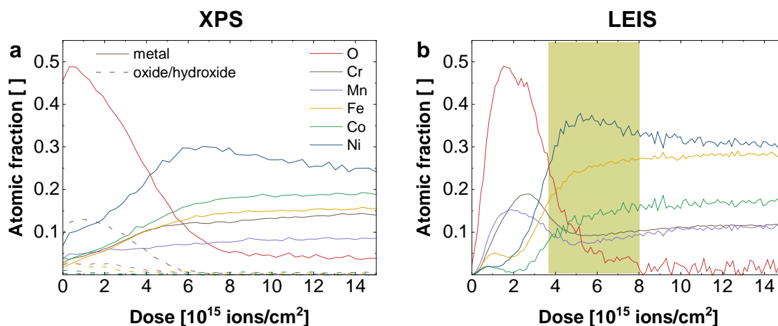
Fig. 3 Comparison of sputter depth profiles on CrMnFeCoNi performed with (a) XPS and (b) LEIS. Depletion zone of Mn and Cr in LEIS is highlighted in yellow. A sputter dose of 2.19 \cdot 10^{15} ions cm -2 corresponds to an estimated depth of 0.6 \pm 0.1 nm (LEIS) resp. 0.7 \pm 0.1 nm (XPS).
