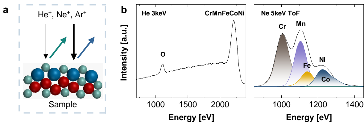
Fig. 2 (a) Working principle of LEIS with indicated pathways of primary (black) and scattered (green, blue) ions. (b) LEIS spectra on the native oxide of CrMnFeCoNi recorded with He + 3 keV (left) and Ne + 5 keV (right), after a sputter dose of 2.19 \cdot 10^{15} ions cm -2
