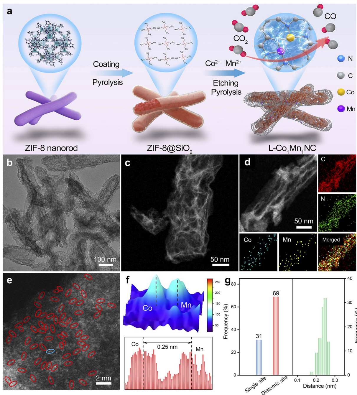
Fig. 1 The morphology and structure characterizations of the L- \text{Co}_1\text{Mn}_1\text{-NC} catalyst. (a) Illustration depicting the PSRR approach utilized in the production of L- \text{Co}_1\text{Mn}_1\text{-NC} catalysts for the \text{CO}_2\text{RR} . (b) TEM image. (c) HAADF-STEM image. (d) EDS mapping (C in red, N in green, Co in blue, Mn in yellow). (e) AC HAADF-STEM image. (f) 3D map of Co/Mn DSs and intensity spacing diagram. (g) The statistical results of atomic site density and distance distribution.
