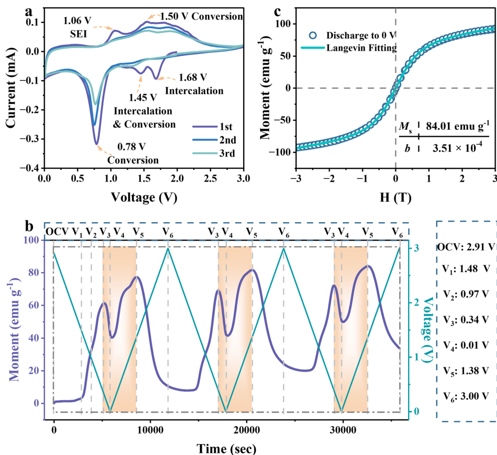
Fig. 2 Electrochemical reaction mechanism of FeOOH LIBs. (a) CV curves for the first three cycles at a scan rate of 0.5 mV s -1 over the voltage range of 0.01–3.0 V. (b) Operando magnetic monitoring followed the voltage range of CV scanning under a magnetic field of 3 T. (c) Magnetic hysteresis loop with the Langevin fitting curve after the first full discharge measured at 300 K.
