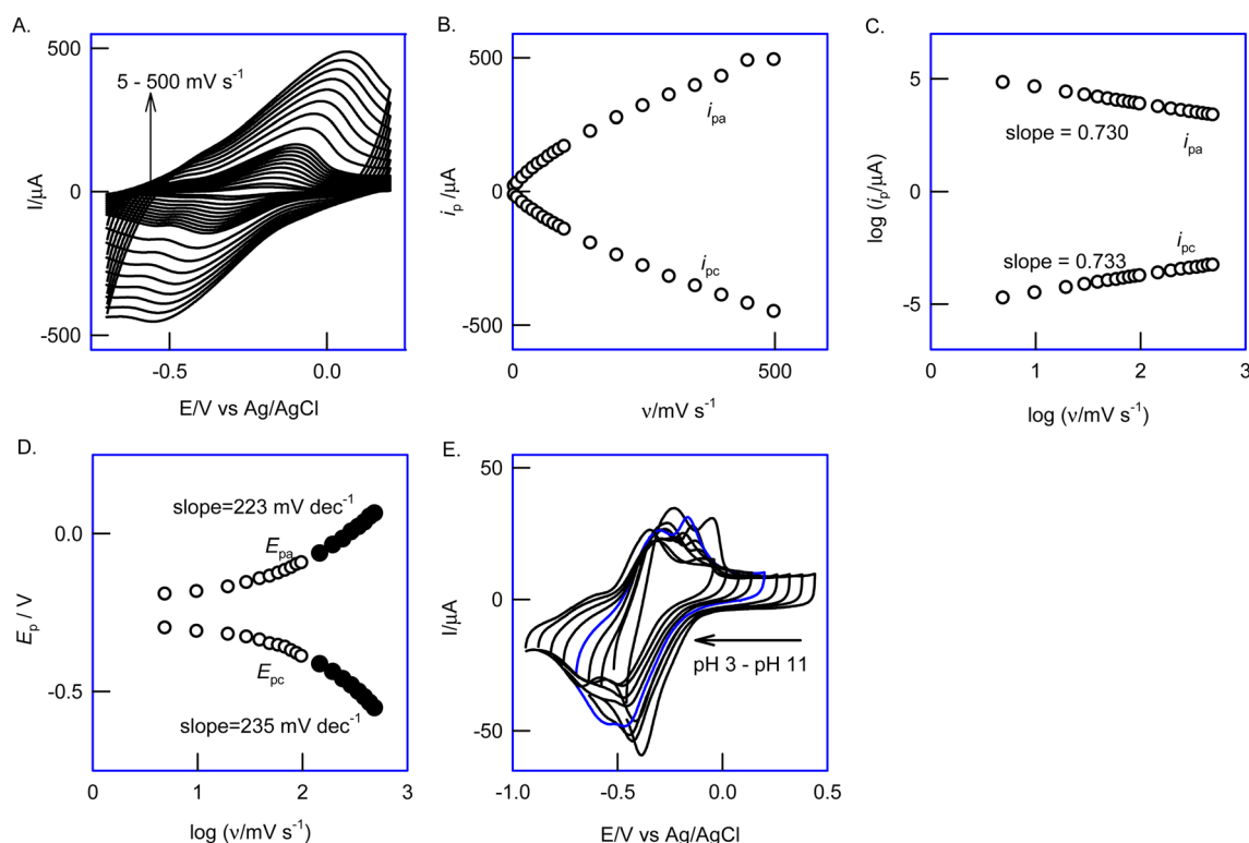
Fig. 2 (A) Effect of scan rate on \text{GCE}/\text{GMC}@{\text{Cu}(\text{BPA})\text{Cl}}_{\text{ads}} -redox from 5 to 500 \text{mV s}^{-1} ; plots of (B) i_p vs. \nu , (C) \log i_p vs. \log \nu and (D) E_p vs. \log \nu ; (E) effect of various pHs (3–11) on \text{GCE}/\text{GMC}@{\text{Cu}(\text{BPA})\text{Cl}}_{\text{ads}} -redox. Electrolyte: in \text{N}_2 purged 0.1 M PBS, pH 7.
