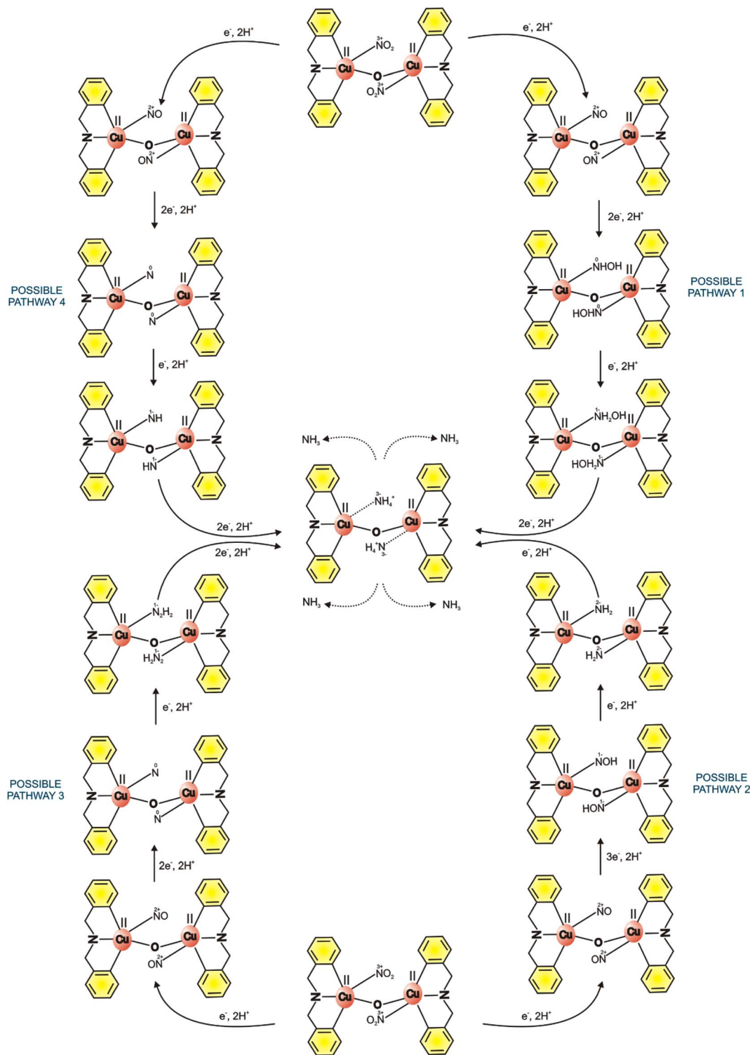
Scheme 3 Possible electrochemical reduction reaction mechanism pathway of GMC@{Cu 2 (μ-O) 2 } on nitrite to form ammonium. The adsorbed NO 2 - is first reduced to NO and its conversion to NH 3 occurs via four pathways: pathway 1: NO → NHOH → NH 2 OH → NH 3 ; pathway 2: NO → NOH → NH 3 ; pathway 3: NO → N → NH 3 ; pathway 4: NO → N → NH → NH 3 . The oxidation states of nitrogen are depicted at each step.
