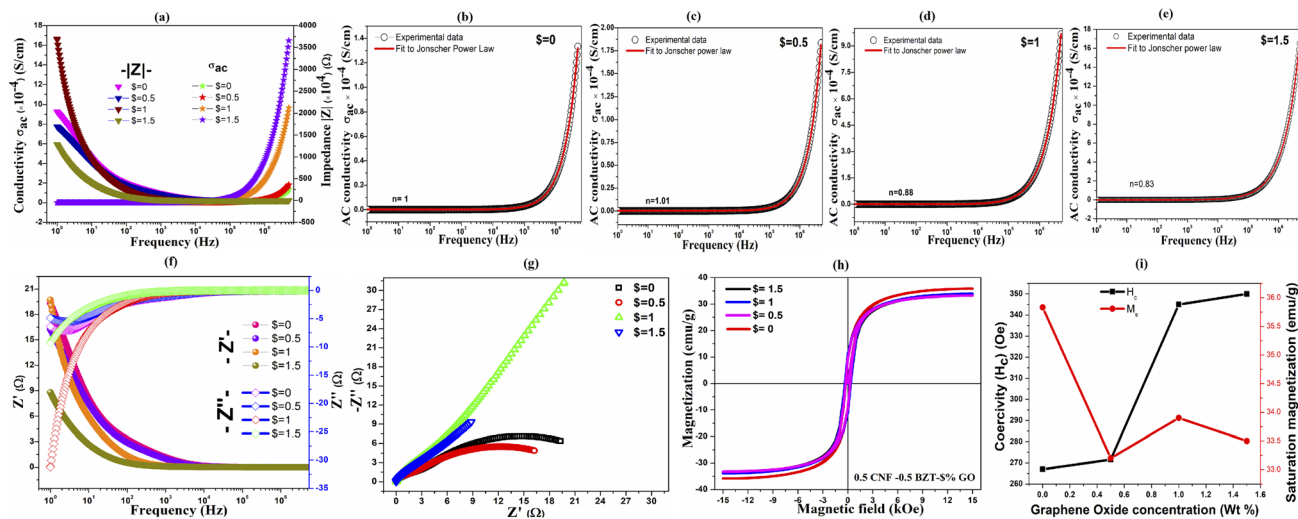
Fig. 6 (a) Conductivity and impedance as a function of frequency for GO decorated magnetolectric composites. (b)–(e) Power law fitting curve for the AC conductivity of 0.5BZT–0.5CNF– S\% GO ( S = 0, 0.5, 1, 1.5 ). (f) Bode plots. (g) Nyquist plot for composites. (h) Composite's magnetization curve as a function of magnetic field. (i) Variation in coercivity and saturation magnetization with GO content in the magnetolectric composite.
