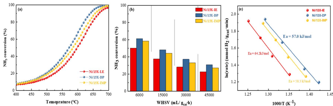
Fig. 8 \text{NH}_3 conversions obtained at (a) WHSV = 30\,000 \text{ mL g}_{\text{cat}}^{-1} \text{ h}^{-1} and 400\text{--}700 \text{ }^\circ\text{C} and (b) WHSV = 6000\text{--}45000 \text{ mL g}_{\text{cat}}^{-1} \text{ h}^{-1} and 550 \text{ }^\circ\text{C} . (c) Arrhenius plots of Ni/13X zeolite catalysts determined over a \text{NH}_3 conversion range of 10–30% at a WHSV of 30\,000 \text{ mL g}_{\text{cat}}^{-1} \text{ h}^{-1} .
