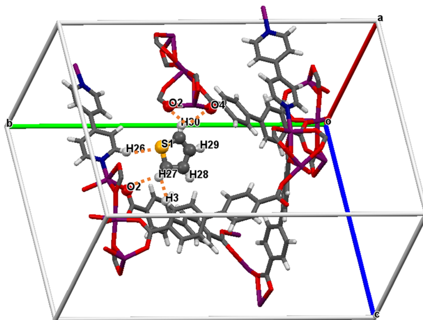
Fig. 9 (a) Packing diagram of BITSH-1 showing thiophene molecules encapsulated inside the pores of the 2-fold interpenetrated structure. C, H, and S atoms are represented in grey, white, and lime colours, respectively. (b) Packing diagram showing interactions between the BITSH-1 MOF structure and hiophene molecule.
