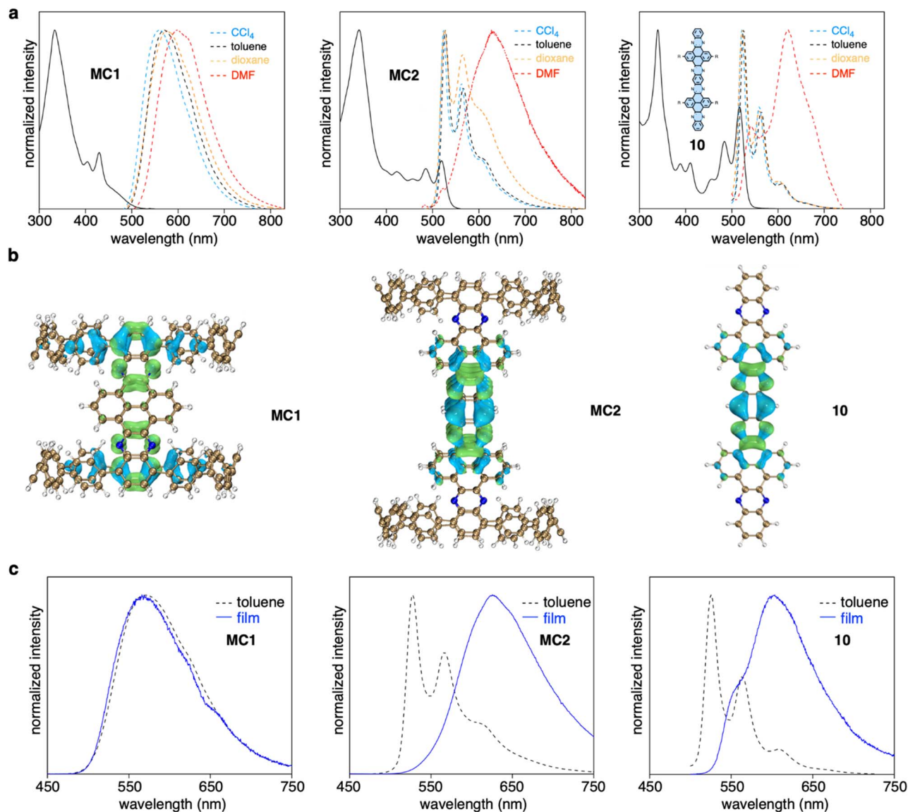
Fig. 4 Photophysical properties. (a) UV-vis absorption (solid line) in toluene and fluorescence (dashed line) spectra of MC1 , MC2 , and 10 . (b) Electron-hole analysis of the S_0 \rightarrow S_1 excitation. Blue and green regions denote hole and electron distributions, respectively (isovalue = 0.001). (c) Fluorescence spectra measured in toluene solution and in the film state.
