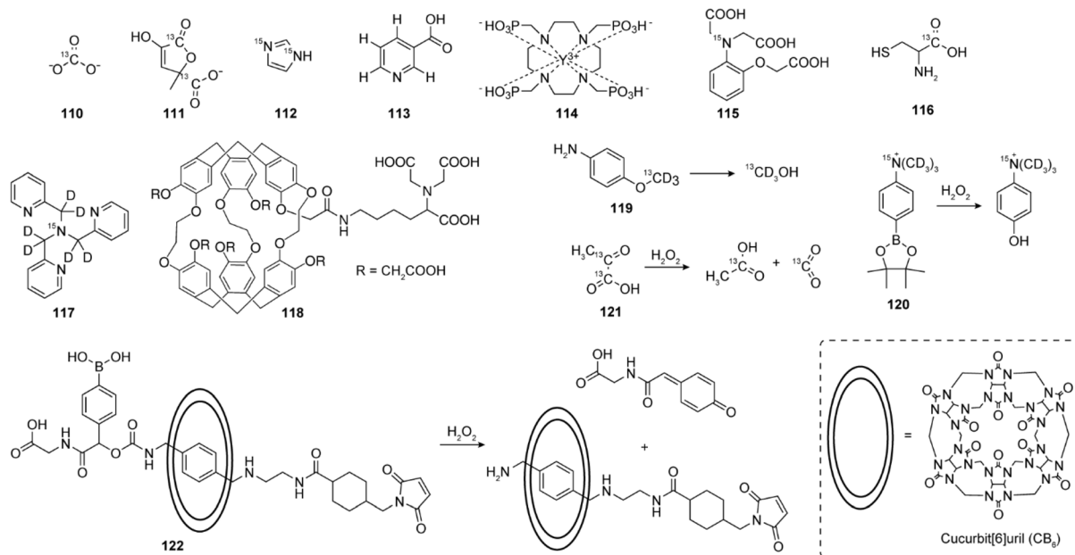
Fig. 14 The representative HP probes that are sensitive to pH ( 110–114 ), Ca(II) ( 115 ), Zn(II) ( 116–118 ), HOCl ( 119 ) and H 2 O 2 ( 120–122 ). These presented probes contain either 3 He, 13 C, 15 N, 89 Y or 129 Xe nuclei to generate HP signal. The following techniques were employed for the signal amplification: dDNP for probes 110–111 , 114–117 and 119–120 ; SABRE for probes 112–113 and 121 ; SEOP for probes 118 and 122 .
