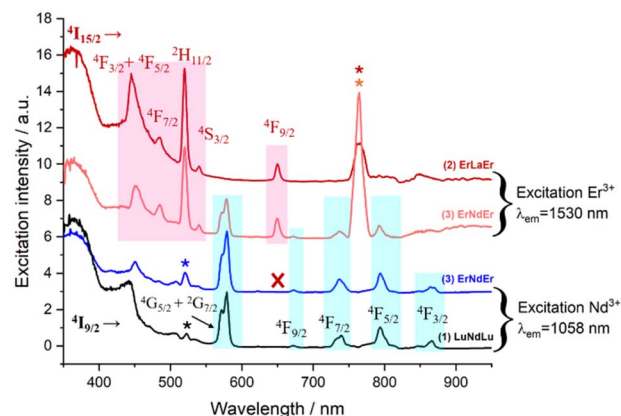
Fig. 8 Excitation spectra of complexes (1) at \lambda_{\text{em}} = 1058 nm (black trace), (2) at \lambda_{\text{em}} = 1530 nm (blue trace) and (3) at \lambda_{\text{em}} = 1058 nm (blue trace) and at \lambda_{\text{em}} = 1530 nm (orange trace) in \text{MeOH-d}_4/\text{DMSO-d}_6 (1 : 1) at 77 K.
