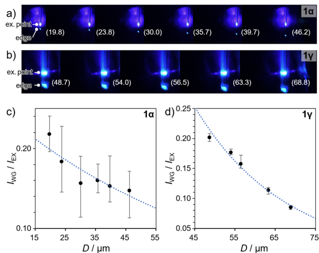
Fig. 8 (a) Fluorescence images of (a) pristine 1α and (b) pristine 1γ with laser excitation ( \lambda_{\text{ex}} = 405 \text{ nm} ) applied at different positions along the long-axis direction. The distance between the excitation and detection points ( D in \mu\text{m} ) is denoted in parentheses. Magnified images are shown in Fig. S22.† (c) Ratios of the emission intensity I_{\text{WG}}/I_{\text{EX}} plotted as a function of D for (c) 1α and (d) 1γ , corresponding to the images in (a) and (b), respectively.
