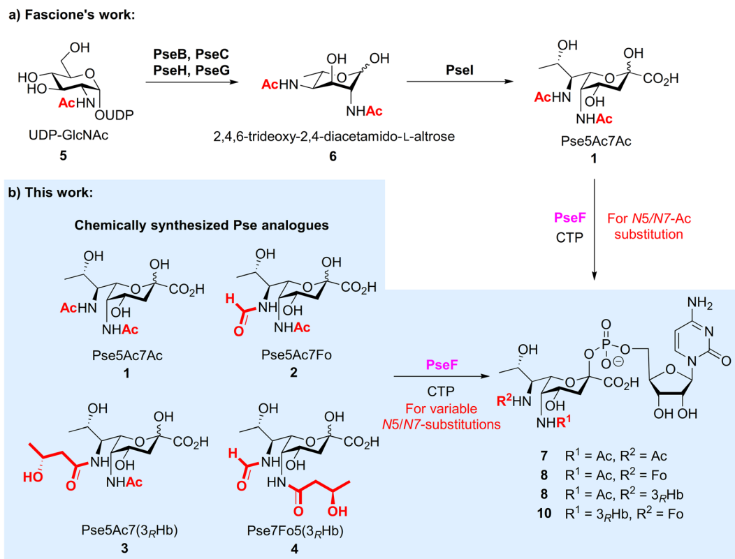
Fig. 2 Enzymatic and chemoenzymatic syntheses of CMP-Pse bearing variable N5/N7 -substitutions. (a) Fascione's enzymatic synthesis of CMP-Pse. (b) Chemoenzymatic synthesis of N5/N7 -modified CMP-Pse in this work.
