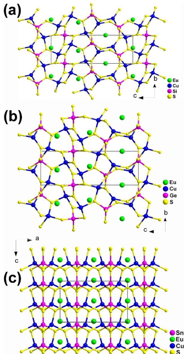
Fig. 3 Structures of (a) EuCu 2 SiS 4 (space group: P3 1 21 ), (b) EuCu 2 GeS 4 (space group: P3 2 21 ), and (c) EuCu 2 SnS 4 (space group: Ama2 ) with the unit cell outlined.
