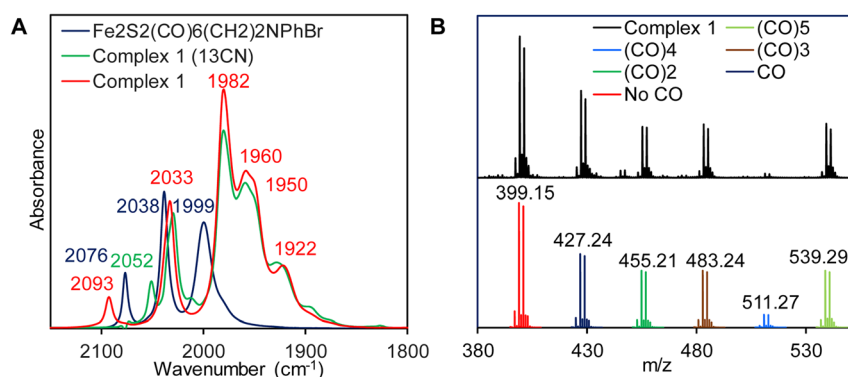
Fig. 1 (A) FTIR spectra for complex 1 (red) & its ^{13}\text{C} analogue (green). The precursor complex is shown in blue (B) (–) \text{ve} ion mode ESI-MS of complex 1 (black) and corresponding simulated spectra with successive five \text{CO} release (bottom).
