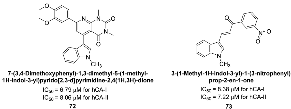
Fig. 25 Chemical structure of compounds 72 and 73 and their IC_{50} values against hCA-I and II.
