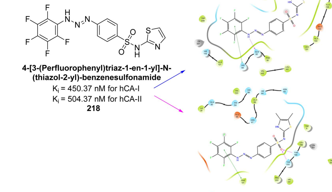
Fig. 79 Chemical structure of compound 218 ; its K_i values against hCA-I and II along with docking images of compound 218 .
