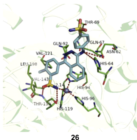
Fig. 16 Chemical structures of compounds 26 and 27 and their IC_{50} values against hCA-IX and docking image of compound 26 against CA-IX (PDB ID: 3IAI).
