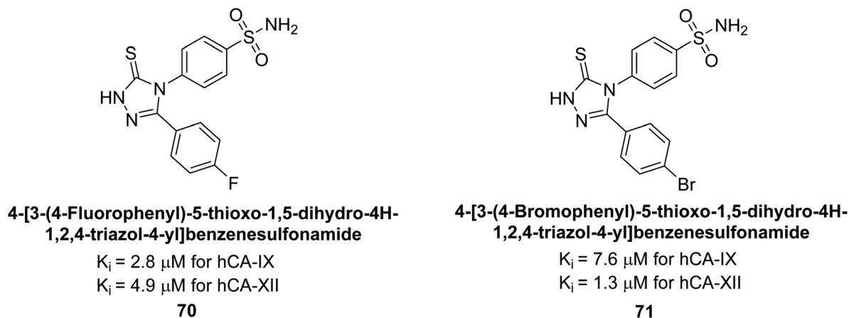
Fig. 24 Chemical structure of compounds 70 and 71 and their K_i values against hCA-XI and XII.
