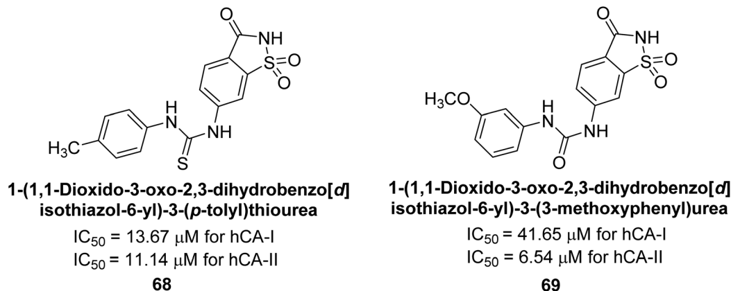
Fig. 23 Chemical structure of compounds 68 and 69 and their IC_{50} values against hCA-I and II.
