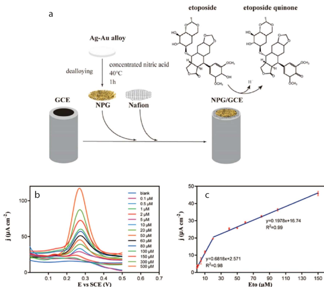
Fig. 3 (a) Shows the fabrication of the sensor (NPG/GCE) and (b) corresponding DPV profile of ETO at an oxidation peak potential of 0.3 V (c) with two linear ranges of 0.1–20 μM and 20–150 μM. 106
