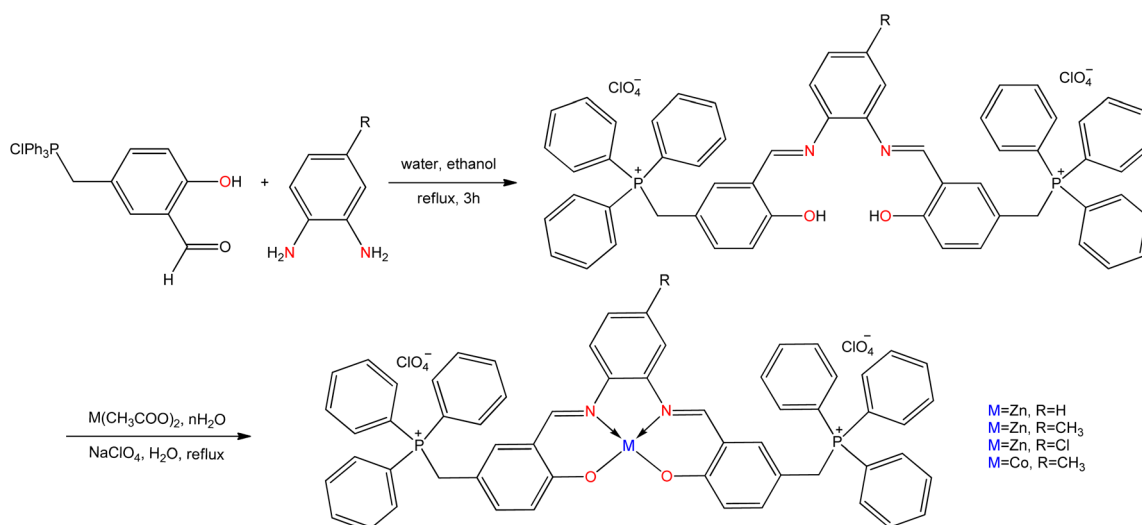
Fig. 16 Synthesis of Schiff base ligand and their metal complexes containing \text{PPh}_3^+ ion.
