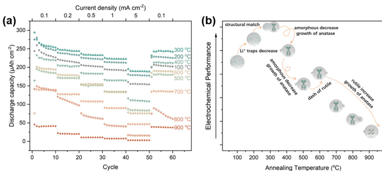
Fig. 7 (a) High rate cycling performance of TNTAs grown for 2 h and annealing at different temperatures. Current density is 0.1\text{--}5\text{ mA cm}^{-2} . (b) Relationship between electrochemical properties and annealing temperature.
