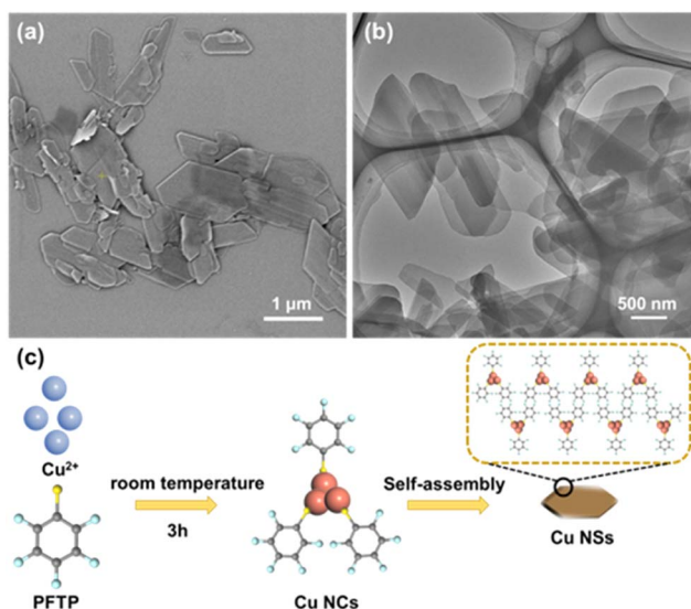
Fig. 1 (a) SEM image of self-assembled Cu NSs. (b) TEM image of self-assembled Cu NSs. (c) Preparation of Cu NSs (schematic).
