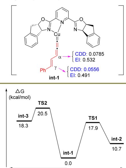
Scheme 4 Preliminary mechanistic studies. BP86/def2tzvp/SMD(methanol)//B3LYP-D3(BJ)/6-31g*/SDD was used for DFT calculations.
