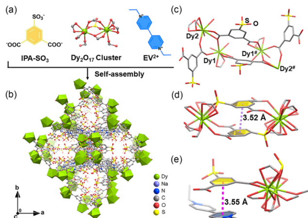
Fig. 1 Crystal structure of RCS-2 : (a) the main building blocks of the structure. (b) 3D framework viewed along the c direction. (c) Coordination spheres of Dy(III) atoms, \text{EV}^{2+} and the ligands. (d) and (e) \pi - \pi stacking interactions (dashed lines) between the ligand and \text{EV}^{2+} . Hydrogen atoms and \text{H}_2\text{O} molecules are omitted for clarity. Symmetry codes: #1 - X , 1 - Y , 1 - Z .
