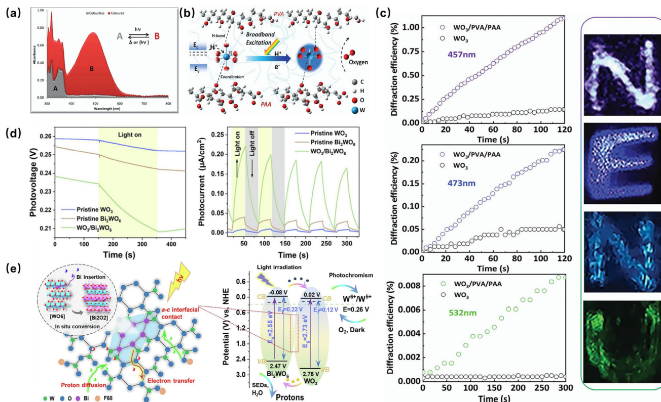
Fig. 3 (a) Photocoloring process. Reproduced with permission. 1 Copyright 2011, Royal Society of Chemistry. (b) Illustration of the photocatalytic reaction mechanism in the \text{WO}_3/\text{PVA}/\text{PAA} hybrid system. (c) Time evolution and color holographic reconstruction of the first-order diffraction efficiency in the recorded configurations at 457 nm, 473 nm and 532 nm for \text{WO}_3 and \text{WO}_3/\text{PVA}/\text{PAA} films. Reproduced with permission. 13 Copyright 2022, Royal Society of Chemistry. (d) Transient photovoltaic and photocurrent responses of pristine \text{WO}_3 , pristine \text{Bi}_2\text{WO}_6 and \text{WO}_3/\text{Bi}_2\text{WO}_6 . (e) Schematic insertion of Bi atoms on the [\text{WO}_6] octahedral framework, \text{WO}_3/\text{Bi}_2\text{WO}_6 photogenerated carrier separation and the photocatalytic color change mechanism. Reproduced with permission. 26 Copyright 2023, Elsevier.
