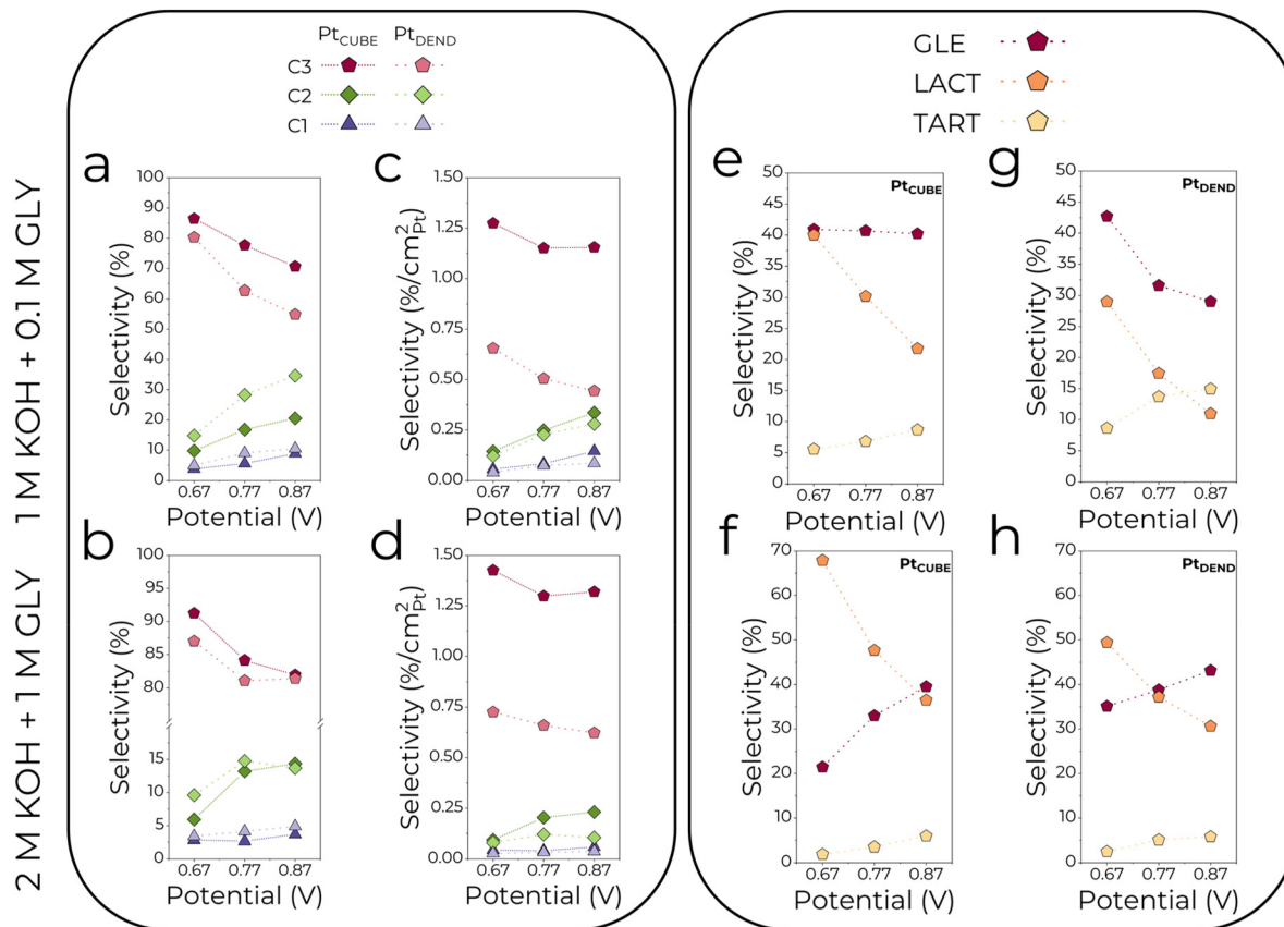
Fig. 4 Selectivity of C3–C1 and individual C3 products as a function of applied potential in (a, c, e and g) 1 M KOH + 0.1 M GLY and (b, d, f and h) 2 M KOH + 1 M GLY electrolytes. Note that (c and d) have different y-axis scales, where the C3–C1 product selectivity is normalised by the aECSA.
