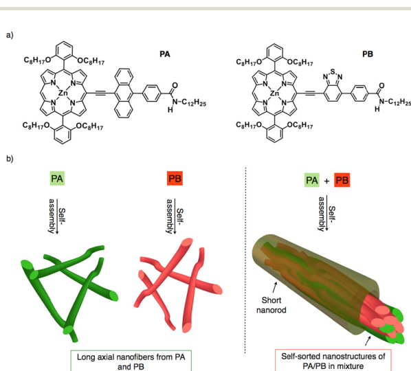
Fig. 1 Molecular structures of Zn(II) metallated porphyrin derivatives comprising (a) anthracene functioning as an electron donor in PA and benzothiadiazole as an electron acceptor in PB . (b) Schematic representation of long axial nanofibers from PA and PB and self-sorted nanostructures embedded in short nanorods from PA + PB upon self-assembly.
