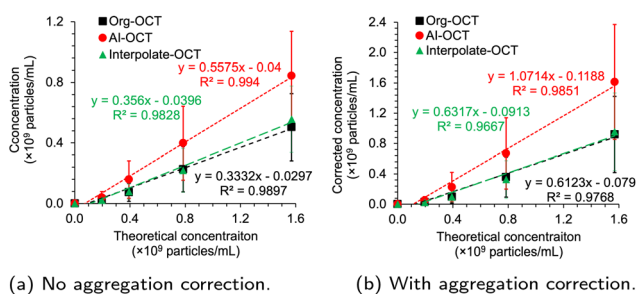
Fig. 3 Correlation of OCT-based particle concentrations with theoretical concentrations and dilutions. The regression line was obtained without the 800 \times diluted sample. (a) No aggregation correction. (b) With aggregation correction.
