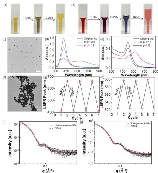
Fig. 1 (a and b) pH-responsiveness of (a) PAA-grafted AgNPs (0.2 mg mL -1 of AgNPs) and (b) PAA-grafted AuNPs. The color change was triggered by adding 0.5 M phosphate acid (H 3 PO 4 ) and sodium hydroxide (NaOH) to tune the solution pH. (c and f) TEM images showing morphologies of PAA-AgNPs at pH values of (c) 2.5 and (f) 12. (d) UV-vis spectra showing the LSPR change of PAA-grafted AgNPs and (e) PAA-grafted AuNPs at different pH values. (g and h) Reversibility of the LSPR shift of (g) PAA-grafted AgNPs and (h) PAA-grafted AuNPs upon titration with H 3 PO 4 and NaOH alternatively. (i and j) SAXS patterns of AuNPs: citrate-capped AuNPs (i) and PAA-grafted AuNPs (j) measured in water.
