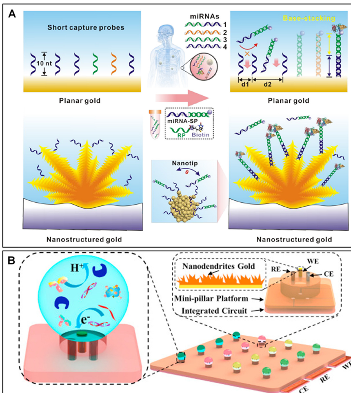
Fig. 7 Electrochemical sensor (A) based on gold nanostructures modified with a short DNA probe for miR21 detection. 91 (B) Open-channel minipillar biosensor for detecting multiple Alzheimer's biomarkers. 94
