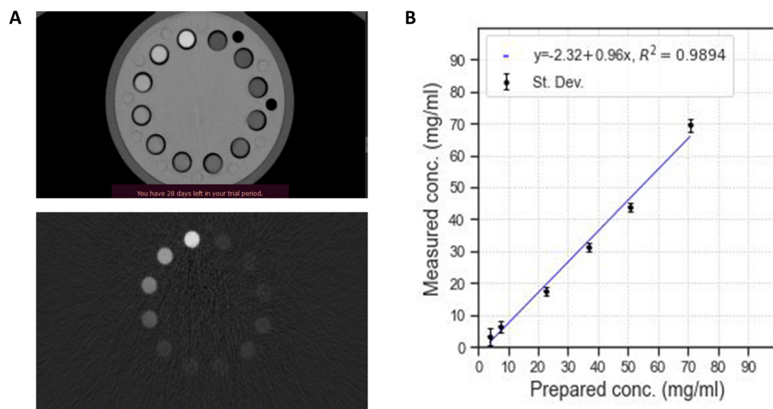
Fig. 4 Imaging and quantification studies on six suspensions of \text{Gd}_{0.90}\text{Tb}_{0.10}\text{F}_3 with concentrations: 3.82 \text{mg mL}^{-1} , 7.50 \text{mg mL}^{-1} , 22.6 \text{mg mL}^{-1} , 36.8 \text{mg mL}^{-1} , 50.9 \text{mg mL}^{-1} , and 70.8 \text{mg mL}^{-1} . (A) Conventional CT imaging of a phantom containing the suspensions (up). Color K-edge imaging of the same phantom (down). The Gd concentration in the suspensions increases clockwise. (B) Correlation between the gadolinium concentrations measured by ICP and by SPCCT.
