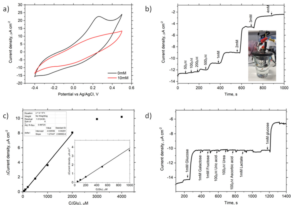
Fig. 5 Electrochemical characterization of the Au/SPhN/PANI/GOx bioelectrode: (a) CV of this bioelectrode without and with 10 mM Glu in PPB pH 7 from -0.4 V to 0.5 V vs. Ag/AgCl at a scan rate of 5 mV s -1 ; (b) the chronoamperometric titration from 50 \mu M to 4 mM of Glu in PPB pH = 7 (inset: photography of the electrochemical cell used in the experiments); (c) changes in currents at -0.4 V vs. Ag/AgCl upon the addition of glucose (inset: data of linear fitting and the change in currents at low Glu concentrations); (d) chronoamperometry after adding interfering reagents at -0.4 V vs. Ag/AgCl.
