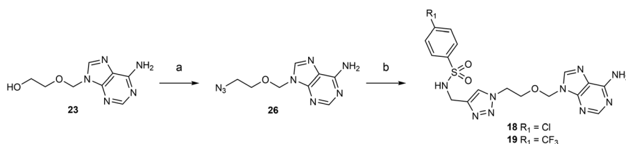
Scheme 3 Synthesis of acyclic adenosine analogues 18–19 . Reagents and conditions: (a) (i) DPPA, DBU, 1,4-dioxane, 25 °C, 16 h; (ii) \text{NaN}_3 , 15-C-5, 100 °C, 4 h, 74%. (b) N -arylsulfonamide- N -propargyl reagents, 11 \text{CuSO}_4 , sodium ascorbate, \text{H}_2\text{O}/\text{dioxane} , 0 °C, 3 h, 74% (for p -Cl), 69% (for p - \text{CF}_3 ).
