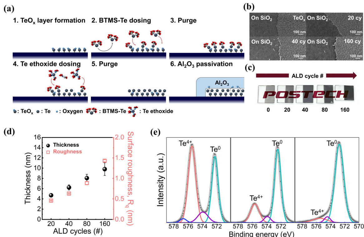
Fig. 1 Defect deficient Te thin film formation via ALD. (a) Schematic process sequence of the ALD process on the seed layer, followed by \text{Al}_2\text{O}_3 passivation. (b) Top-down SEM images of Te deposited on \text{TeO}_x -patterned samples from 0 cycles to 160 cycles. In each of the four sections, the left side of the SEM image displays deposition results on bare \text{SiO}_2 , while the right side shows the results on the region having the seed layer. (c) Photographs displaying the color change at the \text{TeO}_x regions as the cycle of Te deposition increases. (d) Thickness and surface roughness (RMS) of Te including the seed layer, measured by AFM, after 0 to 160 cycles of ALD. (e) XPS spectra of Te 3d_{5/2} , including the \text{TeO}_x layer, the Te layer on \text{TeO}_x , and the \text{Al}_2\text{O}_3 passivated Te layer from left to right.
