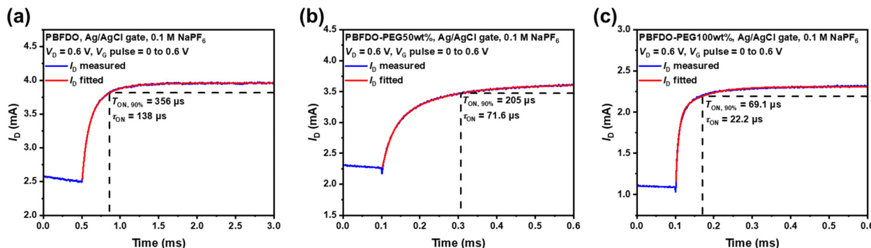
Fig. 5 Temporal response of the drain current ( I_d ) of OECTs with different channel materials. (a) PBFD0; (b) PBFD0-PEG50wt%; (c) PBFD0-PEG100wt%. V_D pulse amplitude = 0.6 V. V_G pulse stated from 0.5 ms (a) or 0.1 ms (b) and (c). T_{ON,90} records the time required for the I_D to grow from the beginning of V_G pulse to 90% of the increase in I_D introduced by V_G pulse. \tau_{ON} is the fitted time constant of the exponential decay curve.
