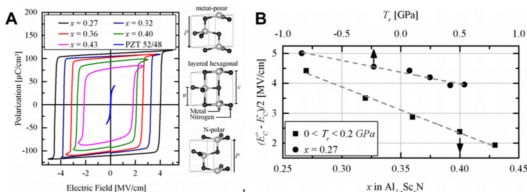
Fig. 4 (A) Ferroelectric Sc_xAl_{1-x}N with Sc contents of 0.27, 0.32, 0.36, 0.40, 0.43 and PZT is the P - E ring of Sc_xAl_{1-x}N . 105 (B) Dependence of the average stress field on the residual stress T_r and Sc content of Al_{1-x}Sc_xN films. Sc content and T_r content vary independently. 105
