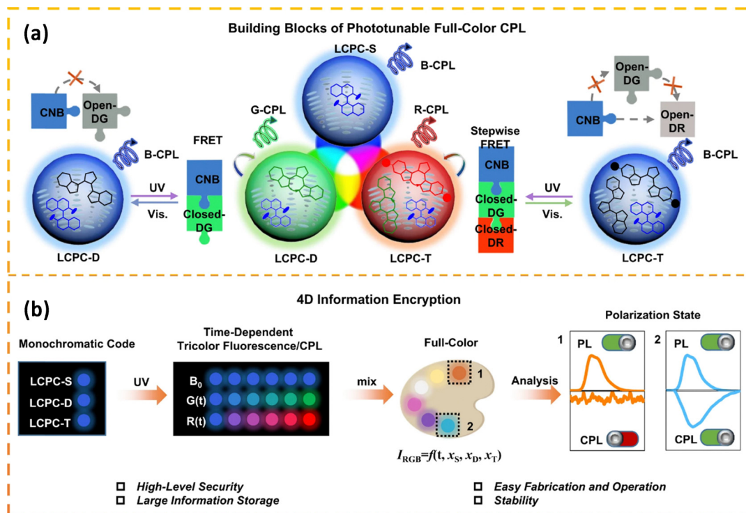
Fig. 7 (a) The light-induced Förster resonance energy transfer (FRET) mechanisms in diverse LCPC components serve as foundational elements for constructing photo-adjustable full-color CPL. (b) The key concept involves designing a 4D information encryption framework, encompassing fluorescence, temporal responsiveness, full-color representation, and CPL attributes. Adapted from ref. 91 Copyright©2023 Springer.
